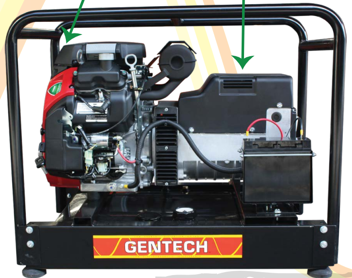
15kVA Honda Generator Model: EP15000HSRE
